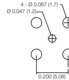
Recommended Mounting Holes
