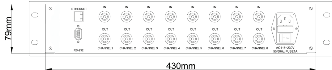
REAR VIEW CHASSIS DEPTH = 350mm
