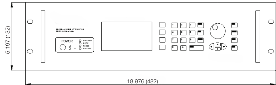
FRONT VIEW
