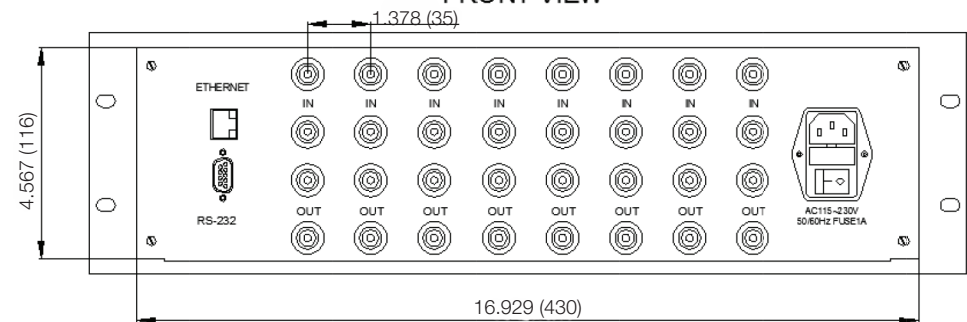
REAR VIEW CHASSIS DEPTH = 18.110 (460)
